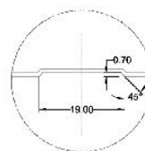
Detail - X-
